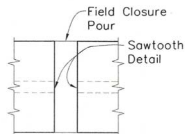
PLAN VIEW GIRDER SPLICE
