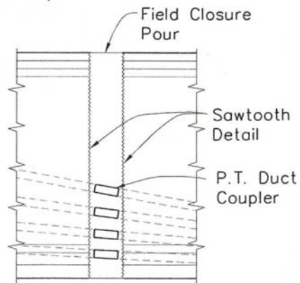
ELEVATION GIRDER SPLICE
