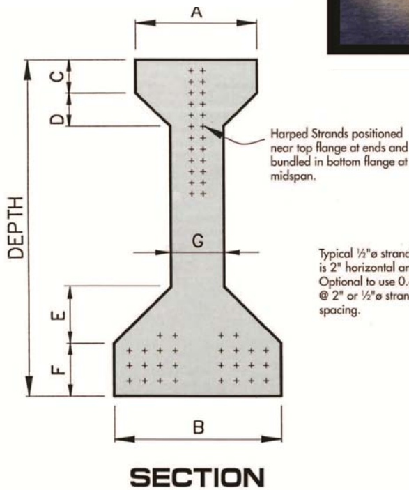
SECTION PROPERTIES
